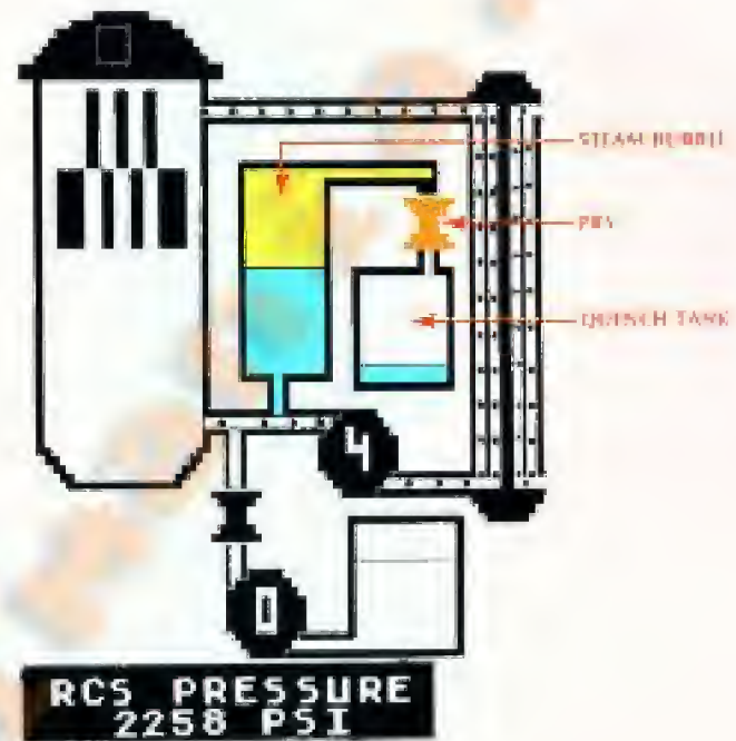
Figure 5. The Pressurizer
